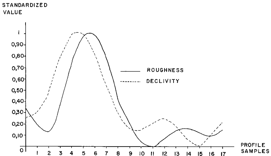
FIGURE III.4 - COMPARISON BETWEEN ROUGHNESS INDEX AND TOPOGRAPHIC TEXTURE, ROUGHNESS INDEX AND DECLIVITY RELATIVE TO THE PROFILES WITH STANDARDIZED VALUES ACQUIRED FROM THE EIGHTH DEGREE TREND SURFACE.
